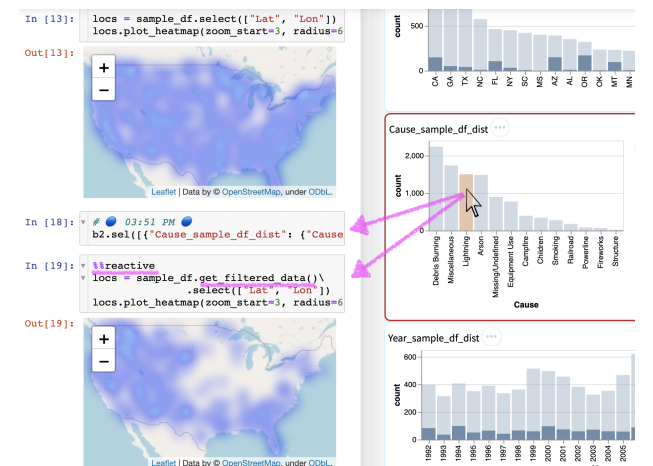
Figure 5. Contrast the top cell, which is static, to the reactive cell below. The reactive cell can be iterated on using interactions.
