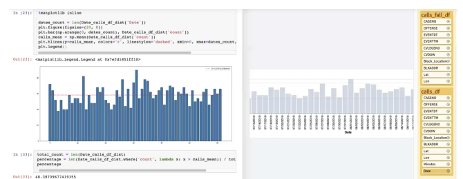
Figure 9. Using code to create a custom plot with the average line in the chart, and computing percentages.
