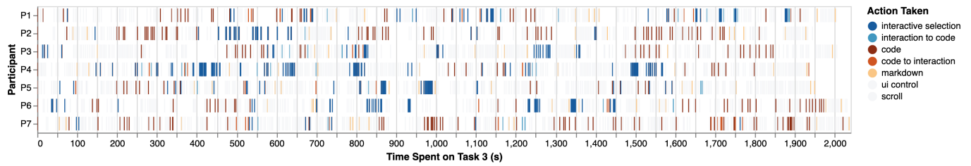
Figure 7. Participants’ interaction traces while working on task 3, an open-ended task to model the dataset. Each participant’s activity is represented by a horizontal strip plot, with participants arrayed down the visualization. Orange colors represents the work done in the code domain, and the blue colors represent the work done in the interactive visualization domain.
