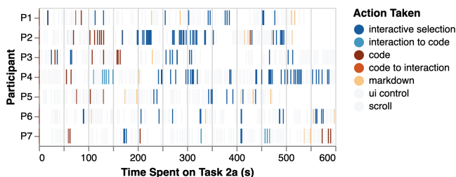
Figure 10. Participants’ interaction traces while working on task 2. To plot the heatmap, all analysts initially interleaved between code and interactions. P3’s gap between 300–400s is when they searched the web for information about the city. P7 used code, interaction, and the get_filtered_data API to inspect whether null values were present.
