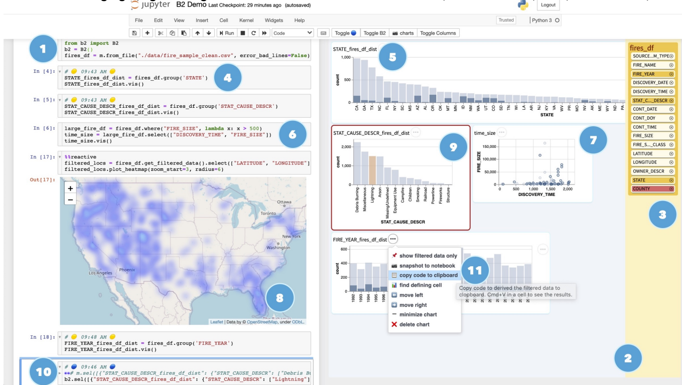
Figure 1. An analyst’s workflow with B2. They start by 1 importing the library which creates 2 a resizable dashboard pane to the right of the traditional notebook. The analyst can 3 click on the columns, which creates 4 code that computes and 5 visualizes corresponding distributions. The analyst can also write 6 a custom data frame query to create 7 the scatter plot. 8 B2’s reactive cells automatically recompute when new interactions occur on visualizations. Interactions involve 9 selections of marks, which link or cross-filter the other visualizations in the dashboard, and are reified in code cells as either 10 an interaction history or by 11 copying their composed predicate definitions.
