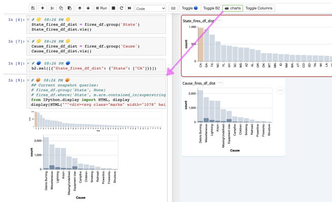
Figure 2. Snapshotting creates a cell in the notebook with an SVG of the visualization, persisting the transient interactive state.
