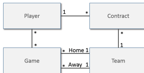
Fig. 3. Simplified database-schema for sports statistics
