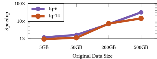
Figure 5: Speedups for different data sizes using two queries (sample fixed to 5GB; Impala).
