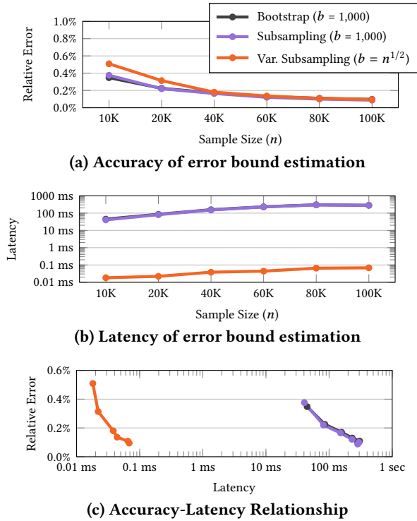
Figure 12: Time-error tradeoff for different sample sizes ( n ).
