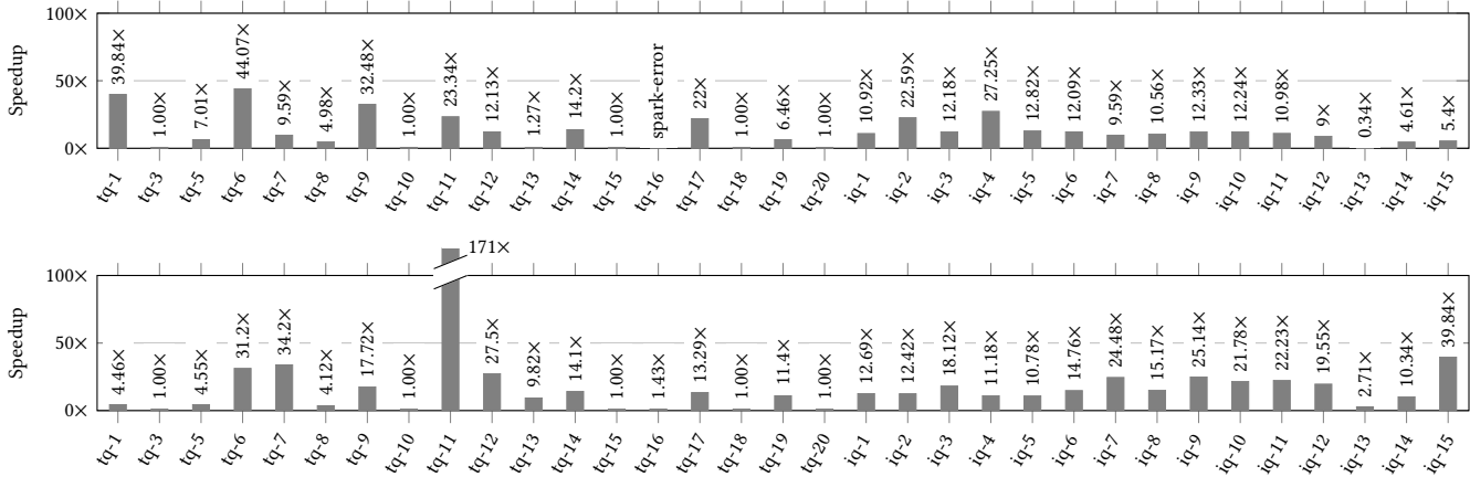
Figure 9: VERDICTDB's speedups for Spark (top) and Impala (bottom).
