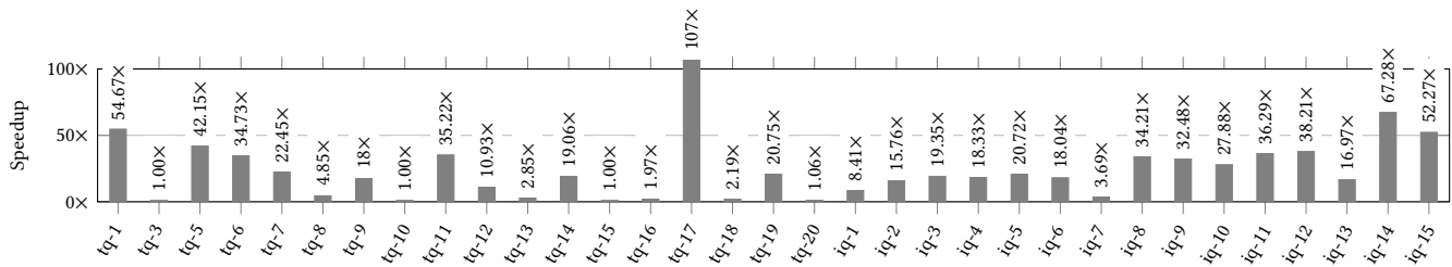
Figure 4: VERDICTDB's speedups for Redshift. Associated errors are in Figure 10. (Spark and Impala deferred to Figure 9.)
