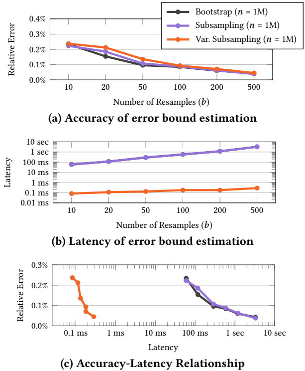
Figure 13: Time-error tradeoff for different numbers of resamples ( b ).
