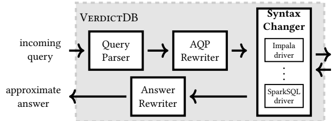
(b) Internal components of VERDICTDB.
